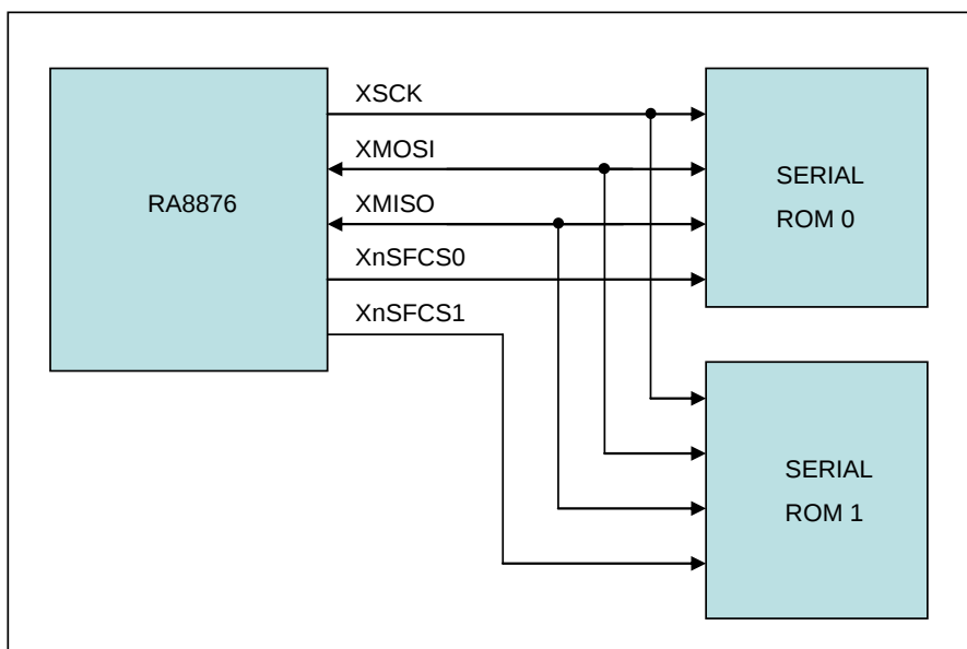
圖 16-3 : RA8876 Serial Flash/ROM System
