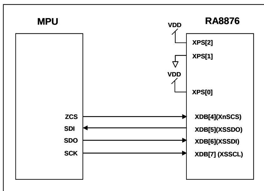
圖 7-13 : The MPU Interface Diagram of 4-Wire SPI
