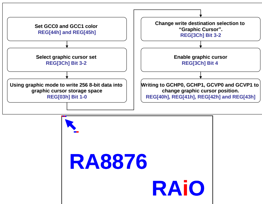
圖 14-21 : The Display with Graphic Cursor
